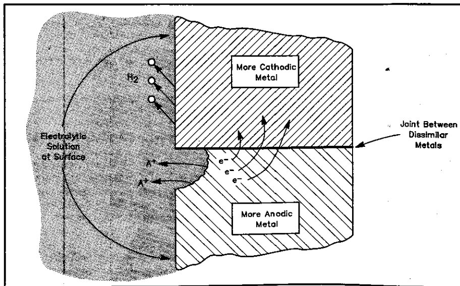
Fig 1—Bimetallic corrosion. When two dissimilar metals are joined in the presence of an electrolyte, the more anodic metal will corrode by releasing positive ions ( A^+ ). This frees electrons ( e^- ) that move across the junction, forming hydrogen bubbles ( H_2 ) at the cathode. This is the same reaction that batteries use, except the electrons flow through a circuit.
