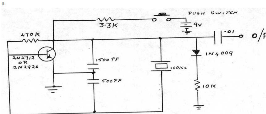
100 Kc CRYSTAL STANDARD
